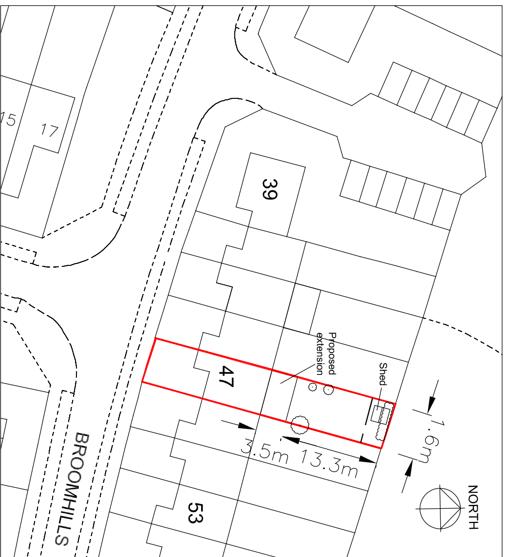
Block Plan 1:500
